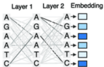
E Transformer
